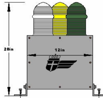
Identification beacon dimensions.
