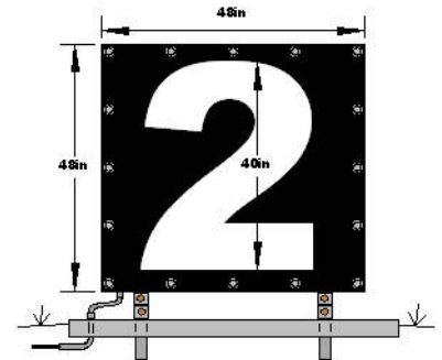
Lighted runway distance remaining sign.
