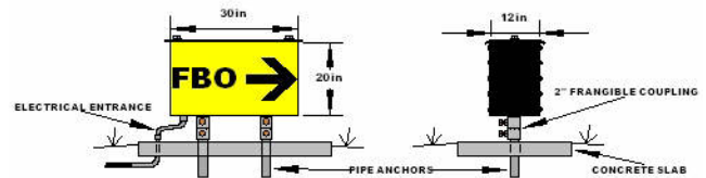
Lighted information sign. 6.6 amp. quartz & 120 volt LED available.
