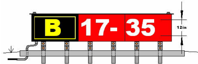
Striplin manufactures signs to FAA L-858 specifications. (Size, style, etc.)
