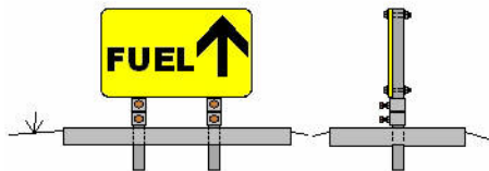
Unlighted reflective information sign with frangible legs.
