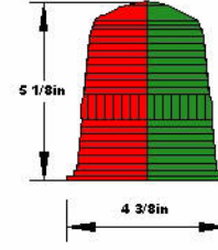
Split color FAA tempered glass lenses for medium intensity fixtures.
