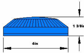
FAA tempered glass lenses for semi-flush heliport fixtures.
