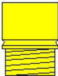
SFC-11 frangible coupling for installing Striplin runway lights on transformer canisters.
