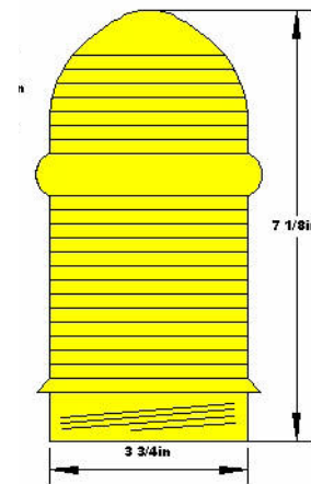
Pyle National style lenses for older obstruction lights and heliport identification beacons.
